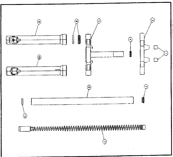
FORCELLA / FRONT FORK R12 COD. 15.03126.000
